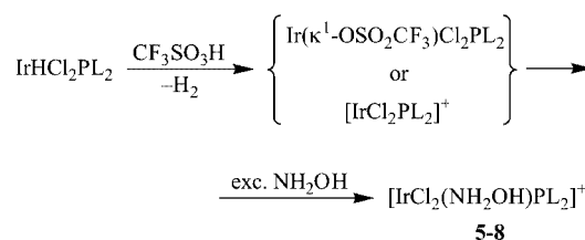
Scheme 3. L = PPh 3 , P = P(OEt) 3 5 , P = PPh(OEt) 2 6 ; L = AsPh 3 , P = P(OEt) 3 7 , P = PPh(OEt) 2 8
