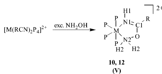
Scheme 5. P = P(OEt) 3 , M = Ru 10 , Os 12 , R = CH 3 a , 4-CH 3 C 6 H 4 b
