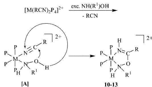
Scheme 7. \text{P} = \text{P}(\text{OEt})_3 , \text{R} = \text{CH}_3, 4\text{-CH}_3\text{C}_6\text{H}_4 , \text{R}' = \text{H}, \text{CH}_3
