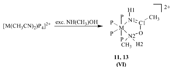
Scheme 6. P = \text{P}(\text{OEt})_3 , M = Ru 11 , Os 13
